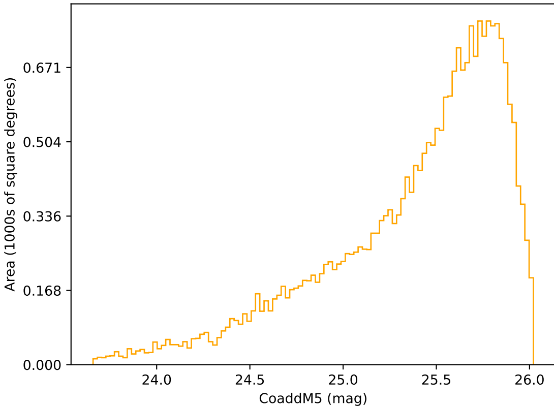
baseline_v3.5_10yrs Yr 3-4 r band: CoaddM5
