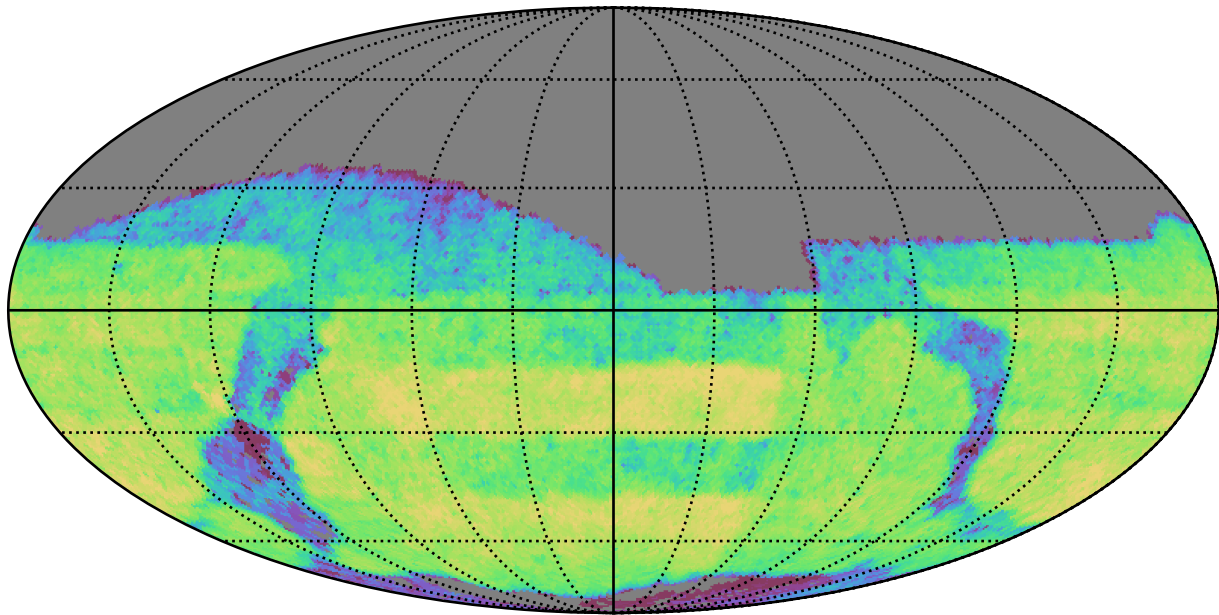
baseline_v3.5_10yrs Yr 3-4 i band: CoaddM5
