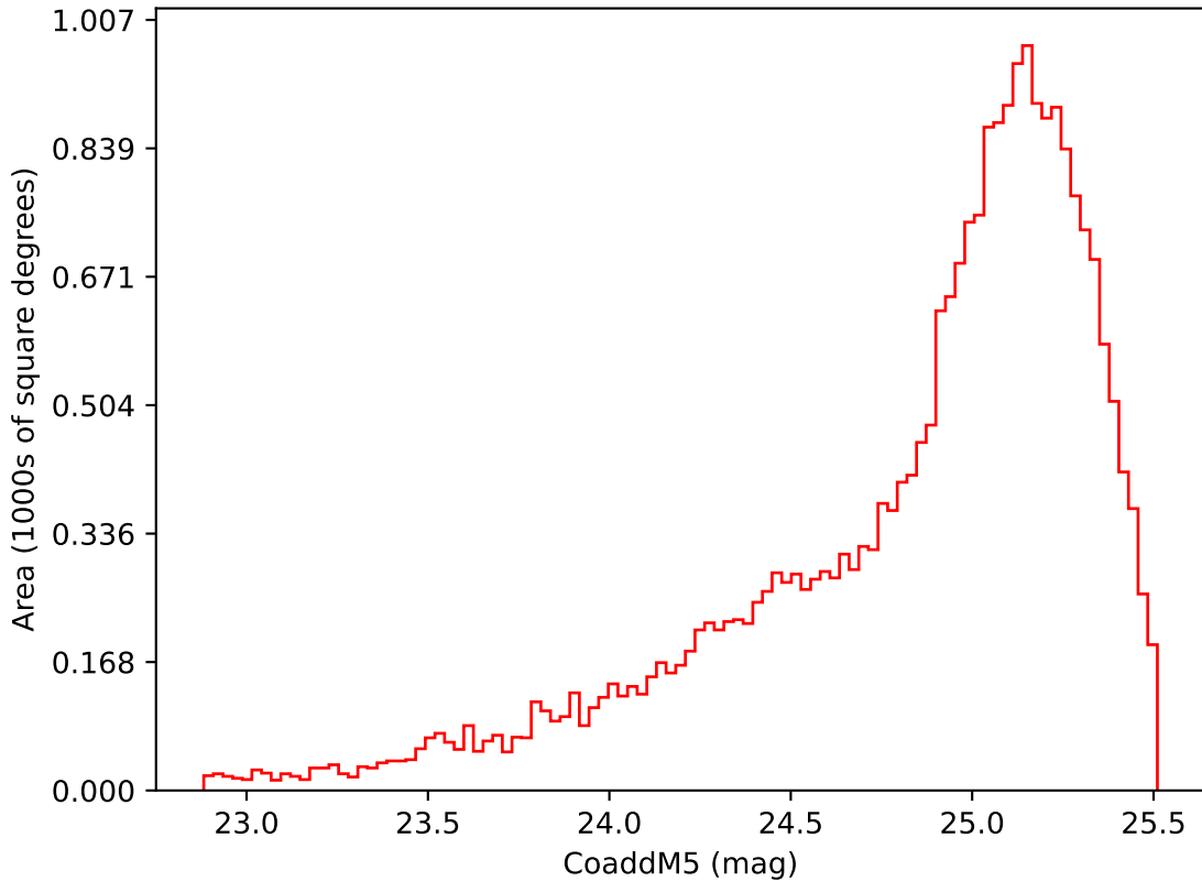
baseline_v3.5_10yrs Yr 3-4 i band: CoaddM5
