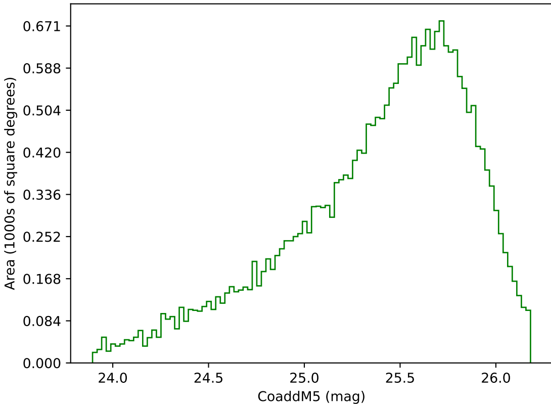
baseline_v3.5_10yrs Yr 3-4 g band: CoaddM5
