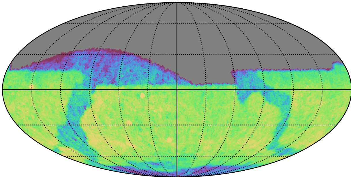
baseline_v3.5_10yrs Yr 1 z band: CoaddM5
