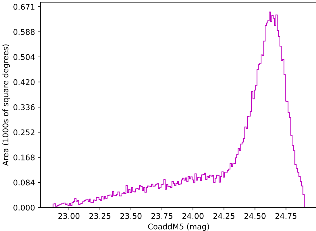
baseline_v3.5_10yrs Yr 1 z band: CoaddM5
