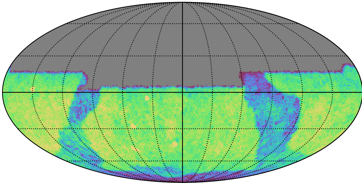
baseline_v3.5_10yrs Yr 1 y band: CoaddM5
