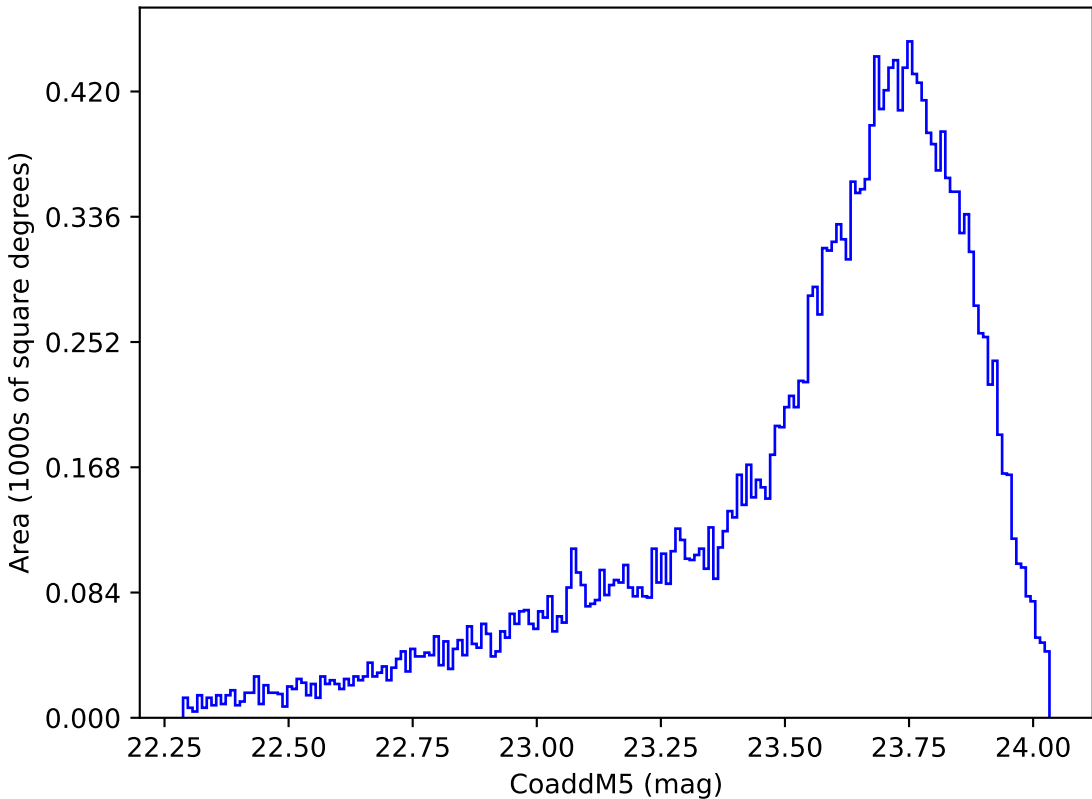
baseline_v3.5_10yrs Yr 1 y band: CoaddM5
