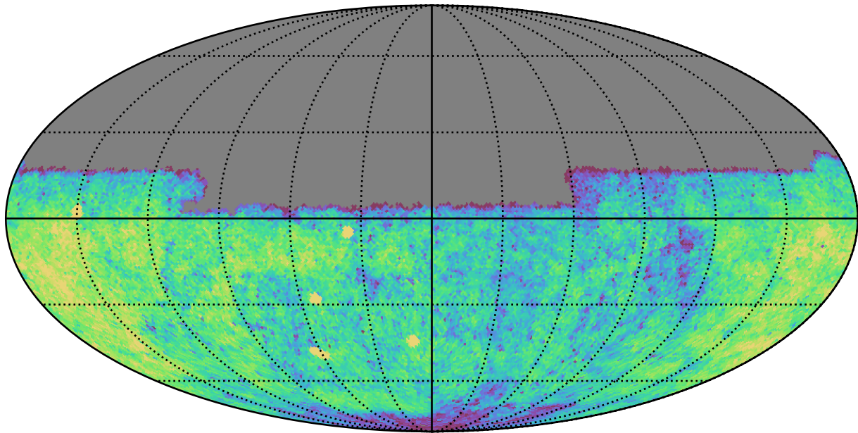
baseline_v3.5_10yrs Yr 1 u band: CoaddM5
