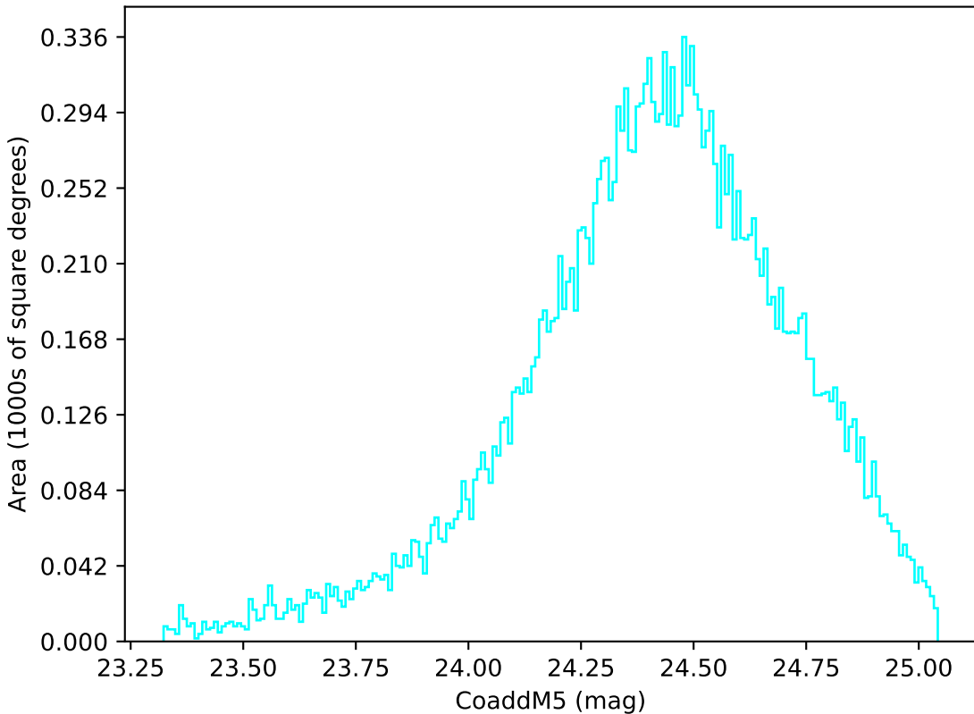
baseline_v3.5_10yrs Yr 1 u band: CoaddM5
