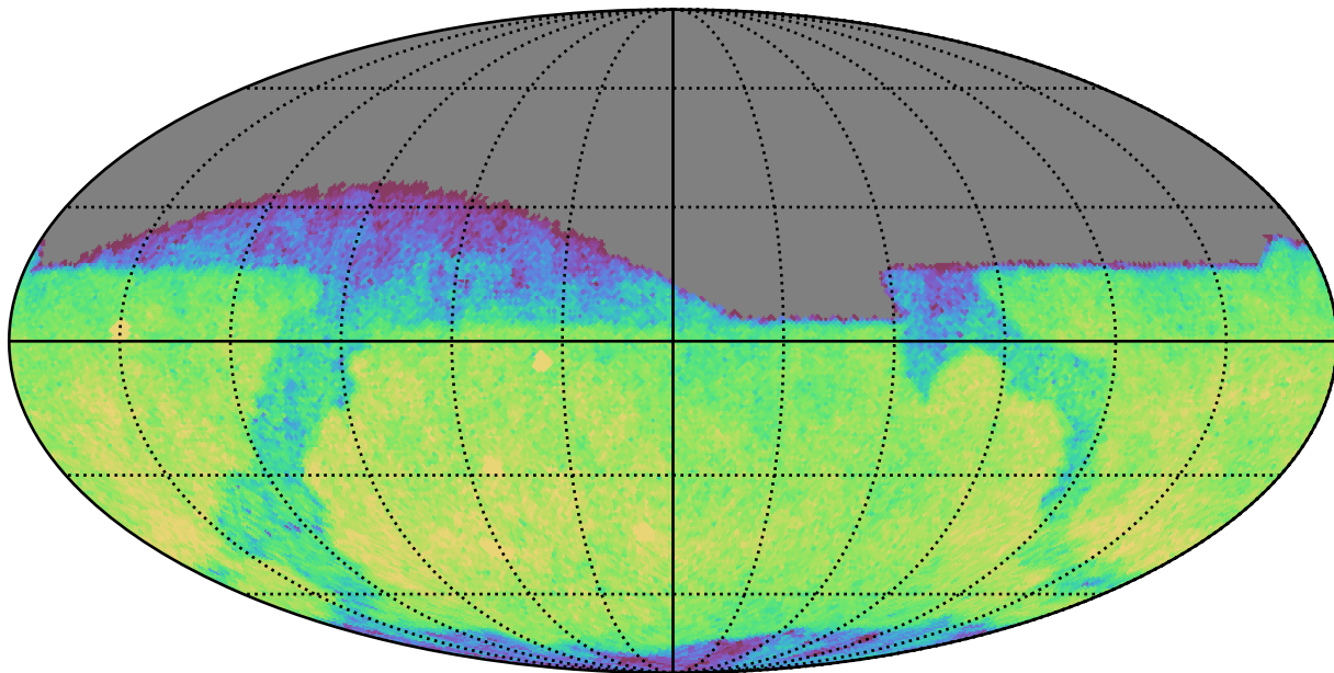
baseline_v3.5_10yrs Yr 1 r band: CoaddM5
