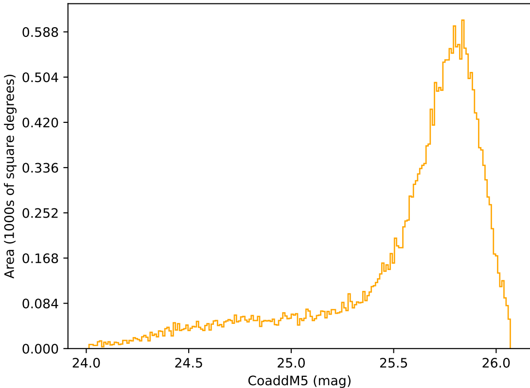
baseline_v3.5_10yrs Yr 1 r band: CoaddM5
