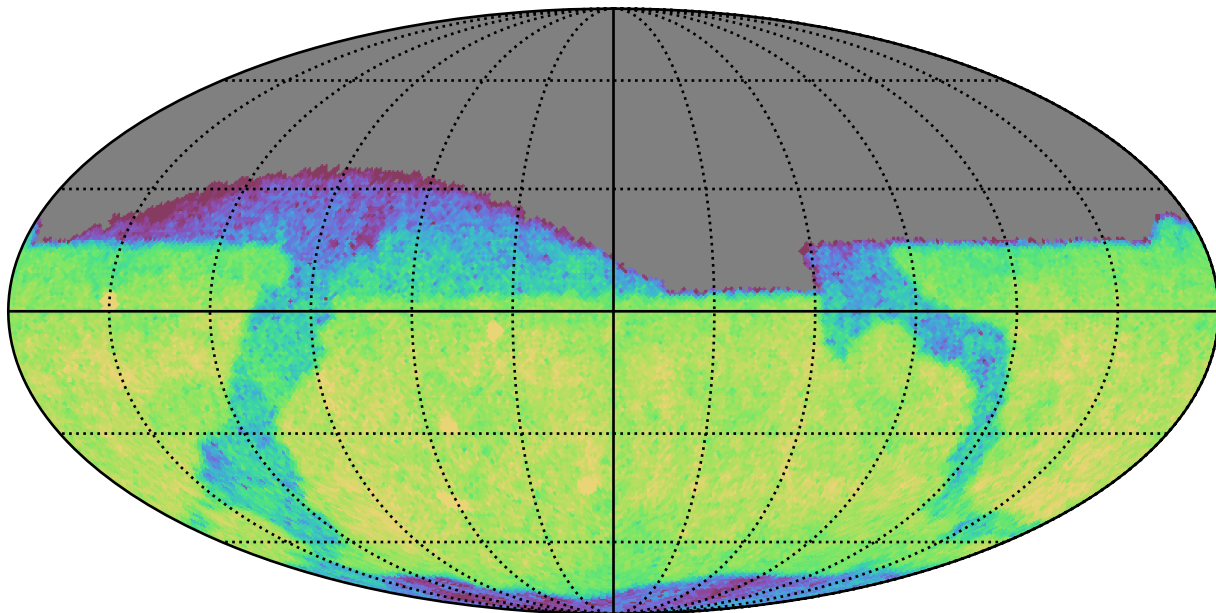
baseline_v3.5_10yrs Yr 1 i band: CoaddM5
