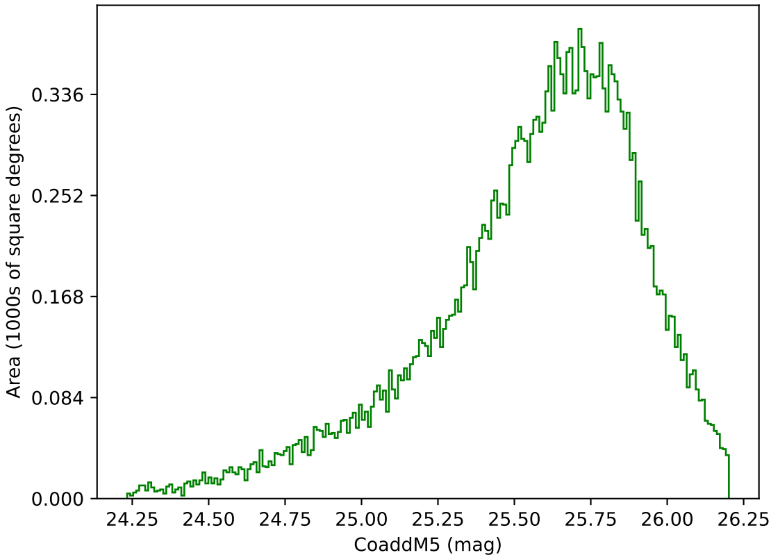
baseline_v3.5_10yrs Yr 1 g band: CoaddM5
