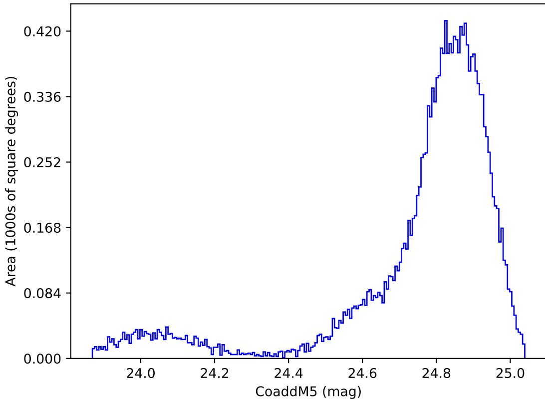
baseline_v3.5_10yrs WFD y band: CoaddM5
