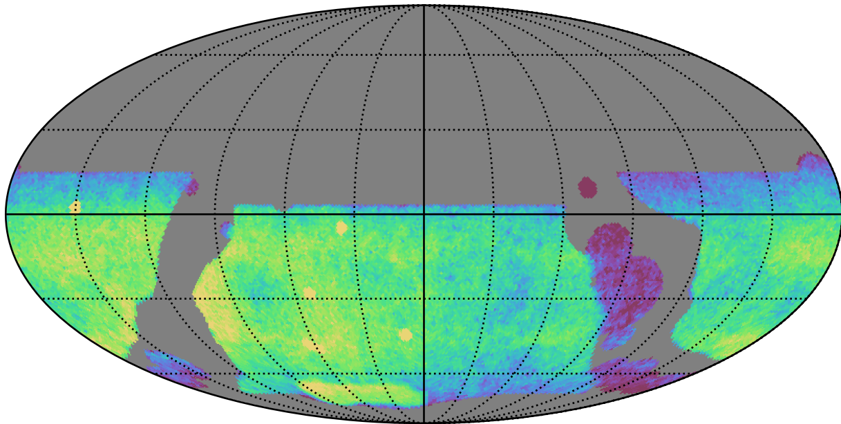
baseline_v3.5_10yrs WFD u band: CoaddM5
