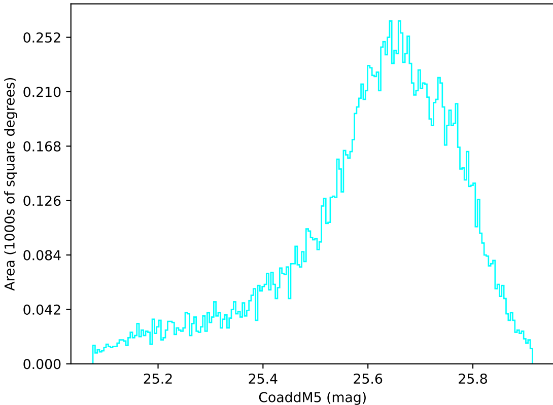
baseline_v3.5_10yrs WFD u band: CoaddM5
