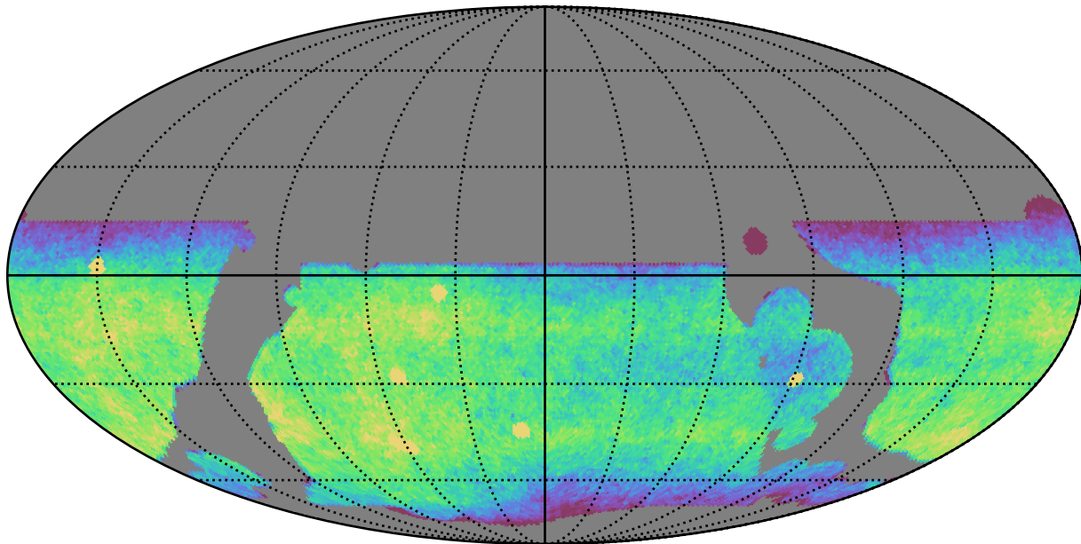
baseline_v3.5_10yrs WFD i band: CoaddM5
