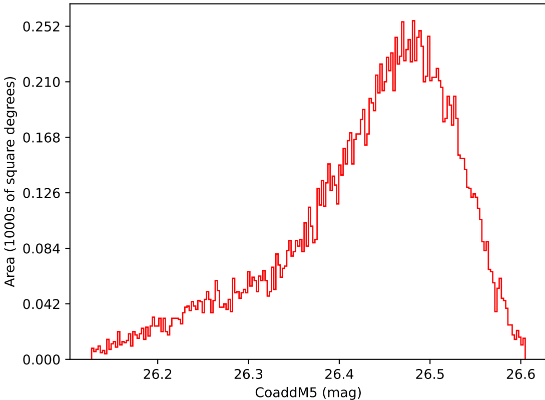
baseline_v3.5_10yrs WFD i band: CoaddM5
