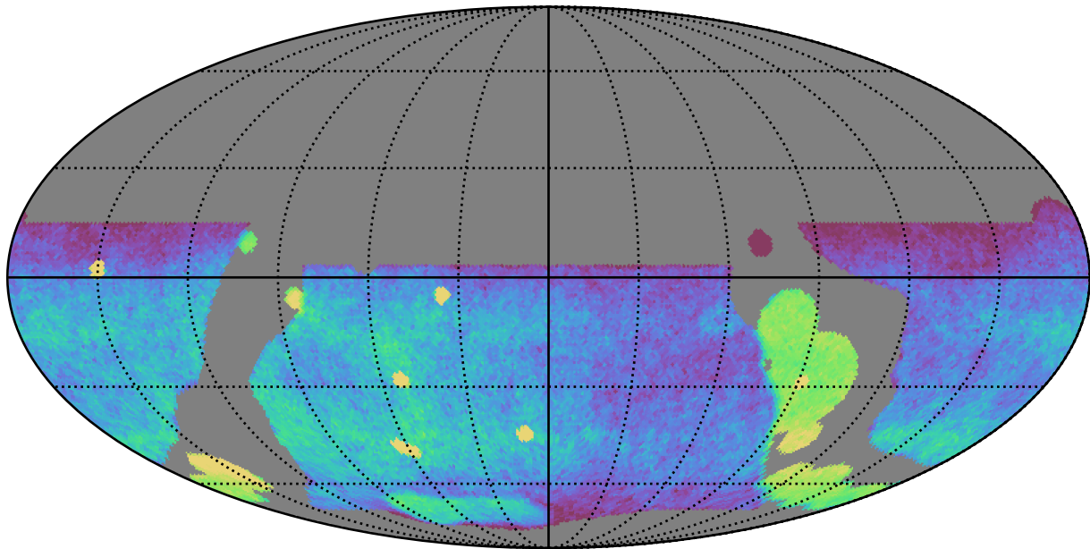
baseline_v3.5_10yrs WFD g band: CoaddM5
