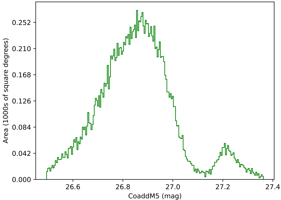
baseline_v3.5_10yrs WFD g band: CoaddM5
