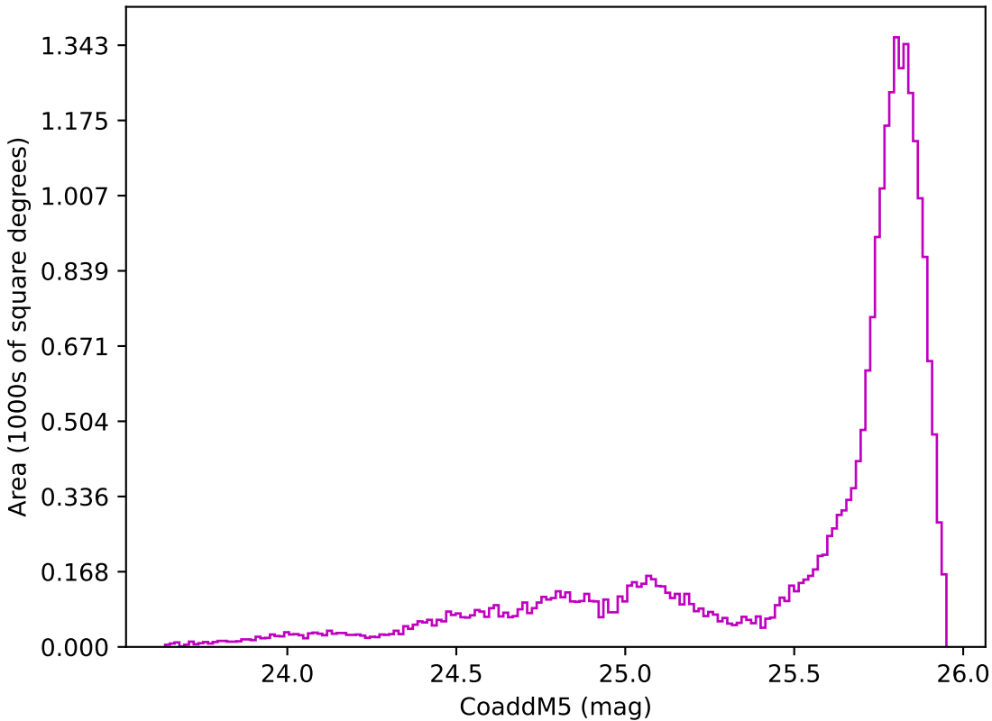
baseline_v3.5_10yrs All sky z band: CoaddM5
