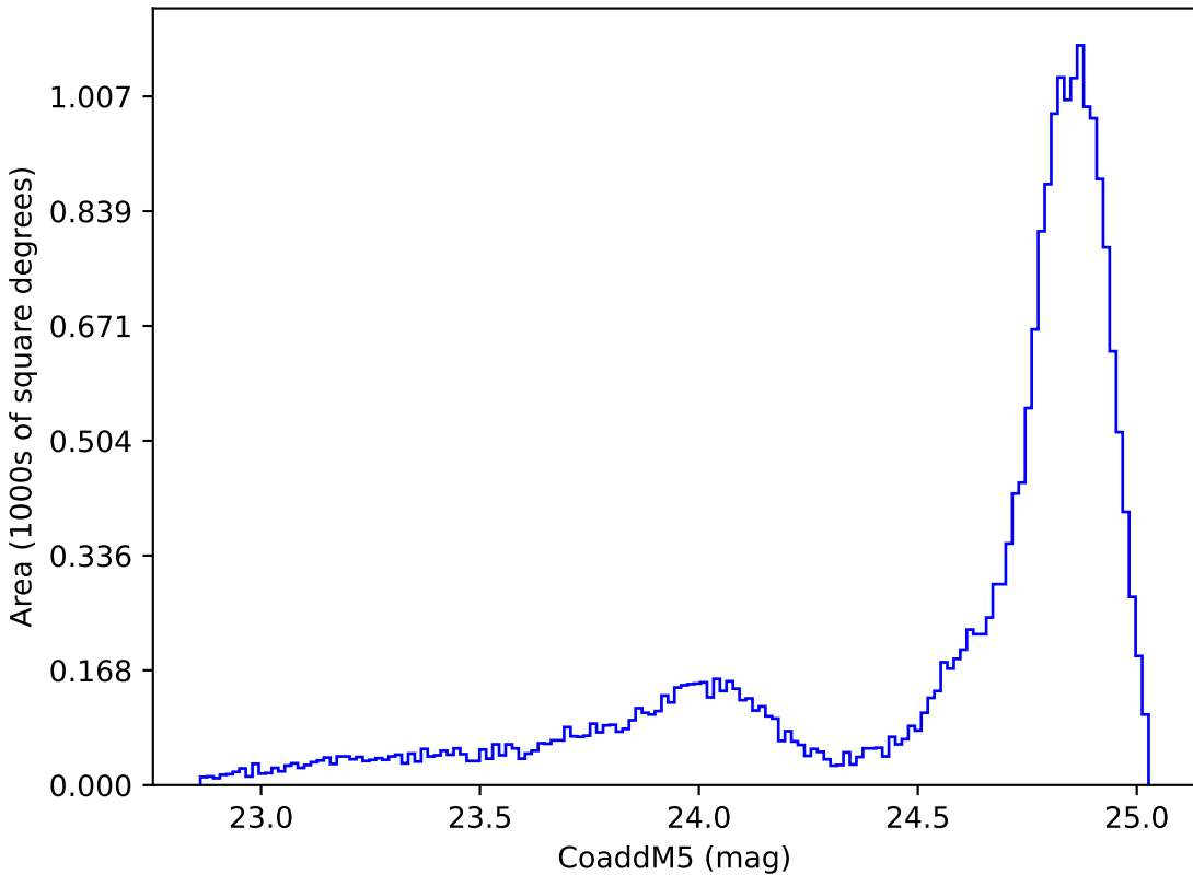
baseline_v3.5_10yrs All sky y band: CoaddM5
