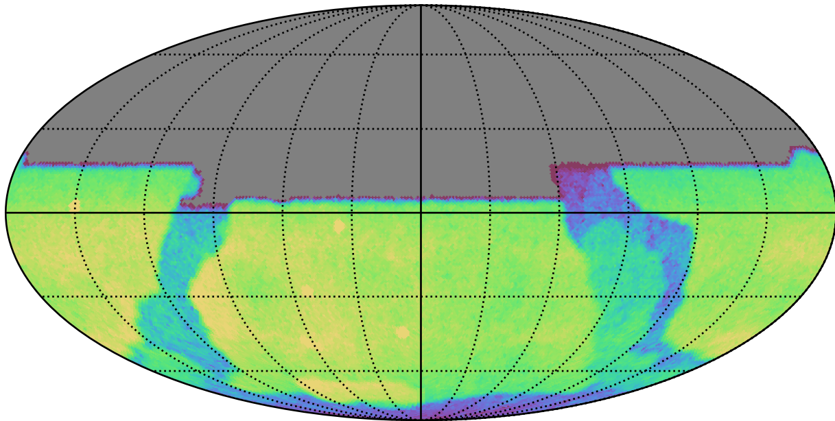
baseline_v3.5_10yrs All sky u band: CoaddM5
