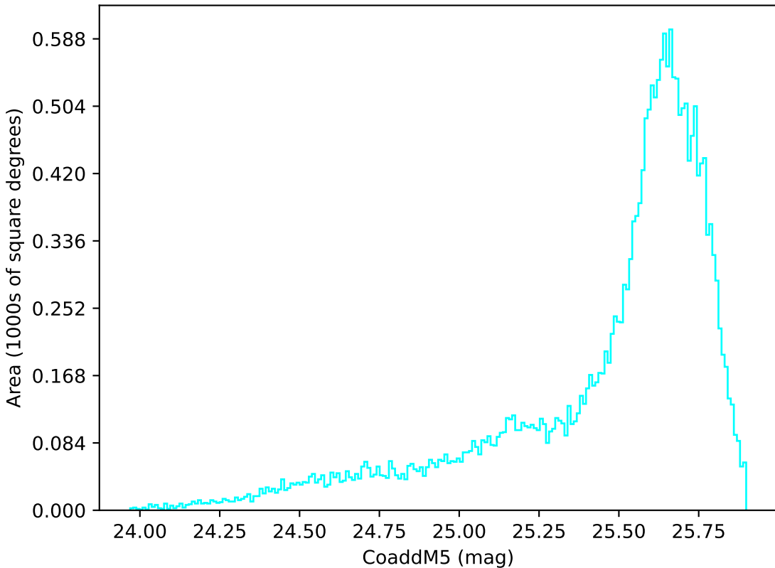
baseline_v3.5_10yrs All sky u band: CoaddM5
