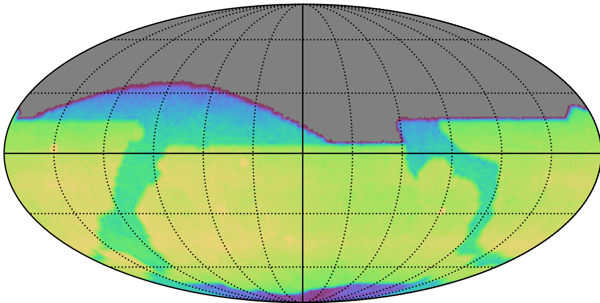
baseline_v3.5_10yrs All sky r band: CoaddM5
