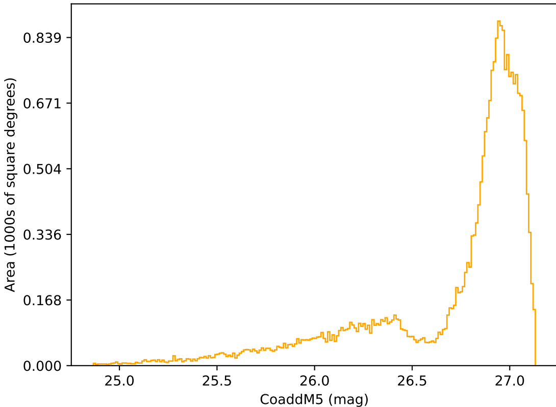
baseline_v3.5_10yrs All sky r band: CoaddM5
