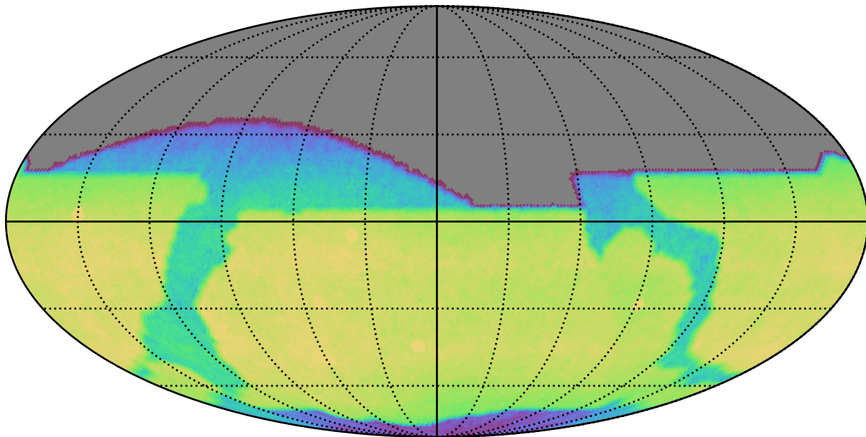
baseline_v3.5_10yrs All sky i band: CoaddM5
