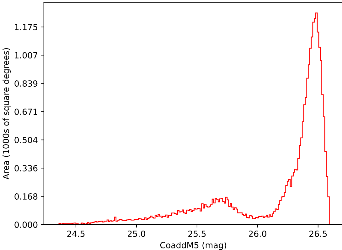
baseline_v3.5_10yrs All sky i band: CoaddM5
