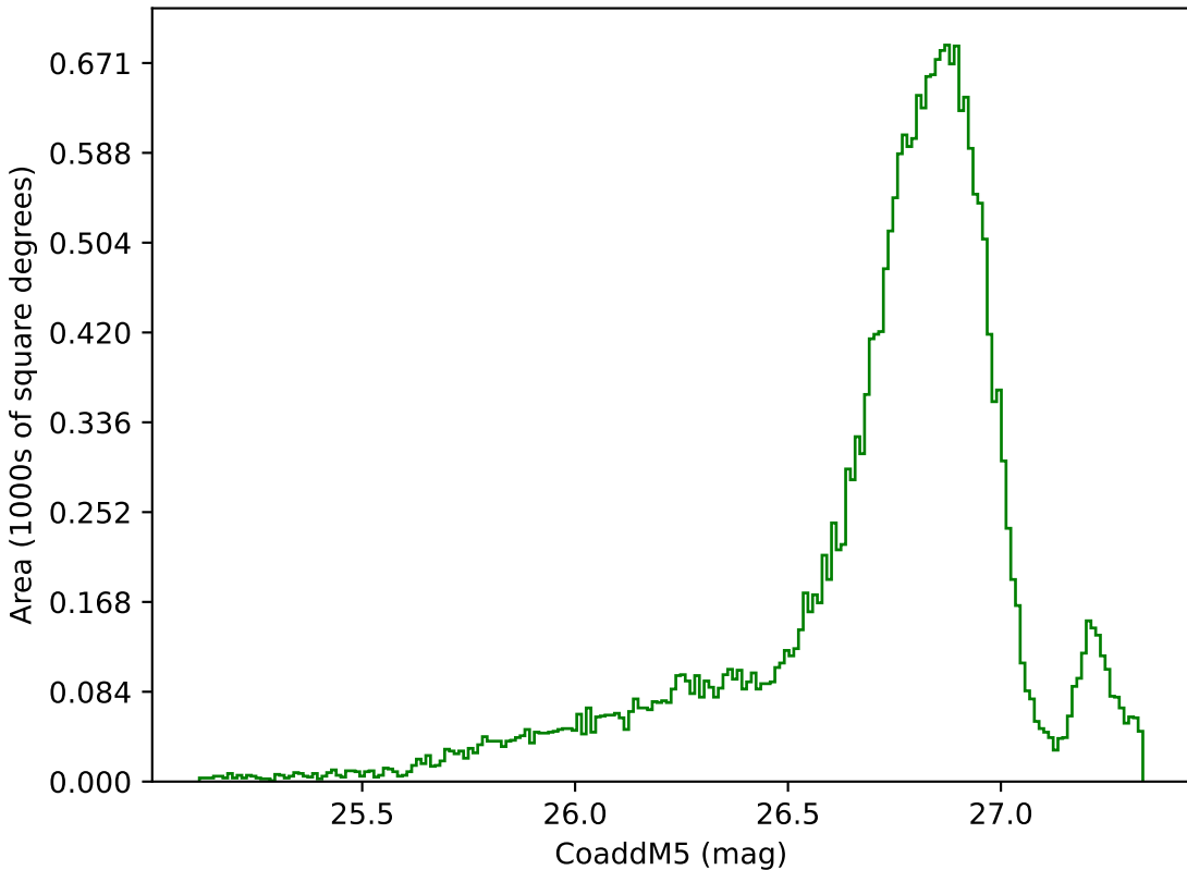
baseline_v3.5_10yrs All sky g band: CoaddM5
