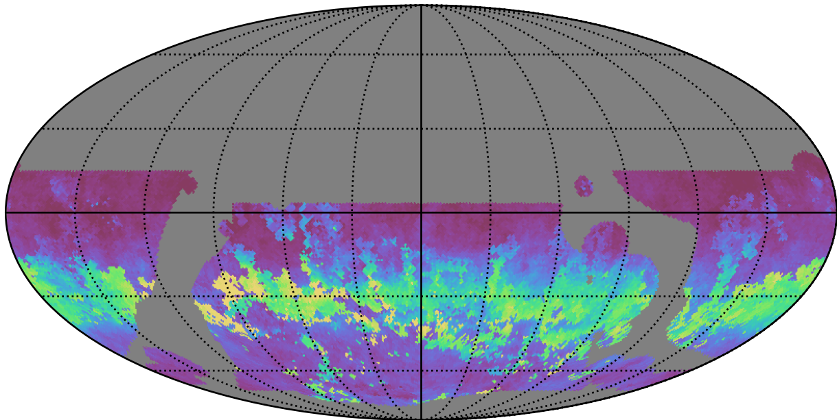
baseline_v3.5_10yrs WFD z band: AngleRms rotSkyPos
