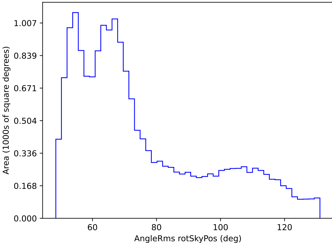
baseline_v3.5_10yrs WFD z band: AngleRms rotSkyPos
