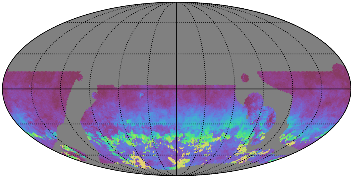
baseline_v3.5_10yrs WFD y band: AngleRms rotSkyPos
