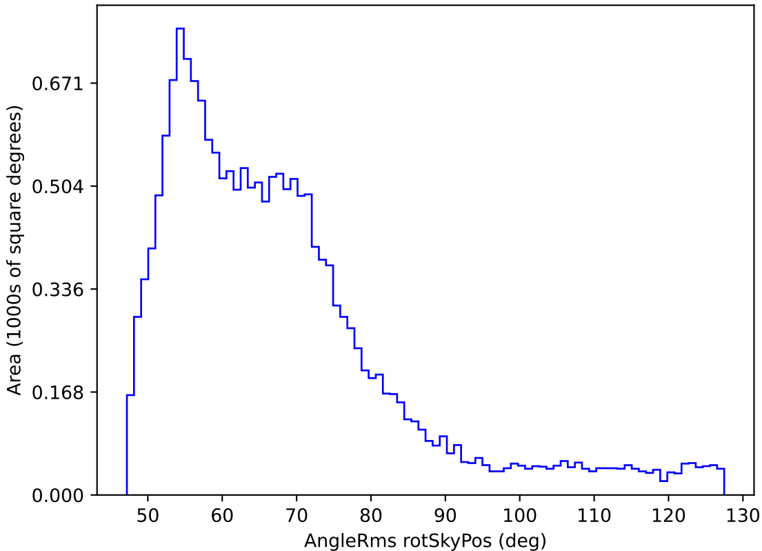
baseline_v3.5_10yrs WFD y band: AngleRms rotSkyPos
