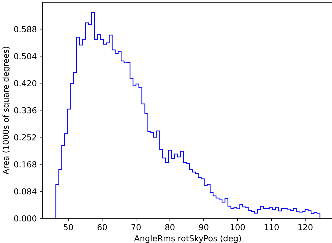
baseline_v3.5_10yrs WFD u band: AngleRms rotSkyPos
