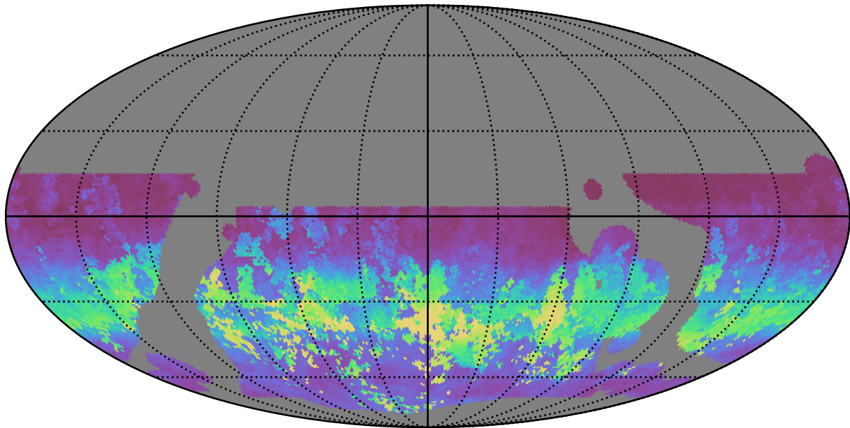
baseline_v3.5_10yrs WFD r band: AngleRms rotSkyPos
