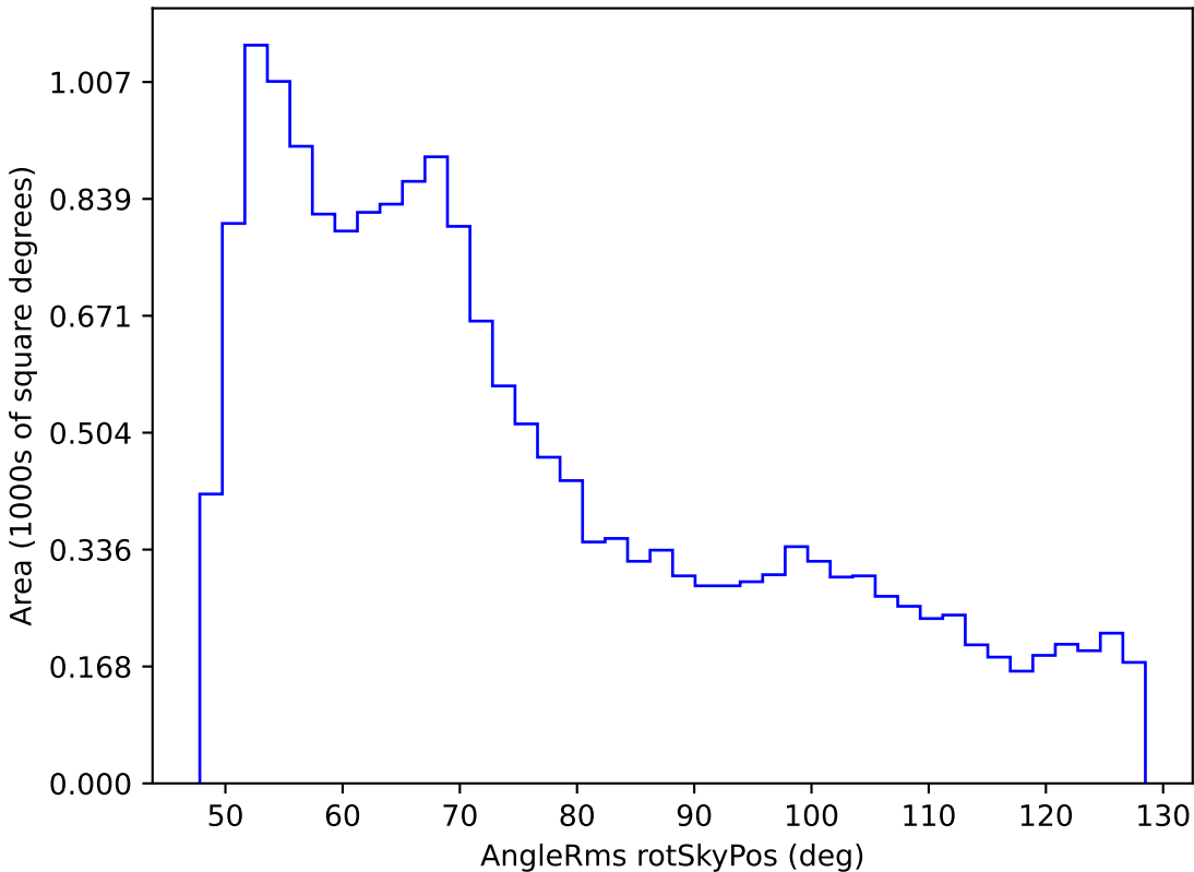
baseline_v3.5_10yrs WFD r band: AngleRms rotSkyPos
