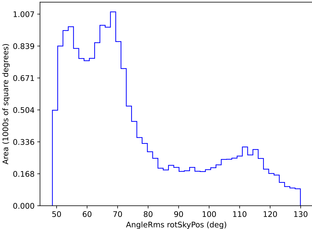
baseline_v3.5_10yrs WFD i band: AngleRms rotSkyPos
