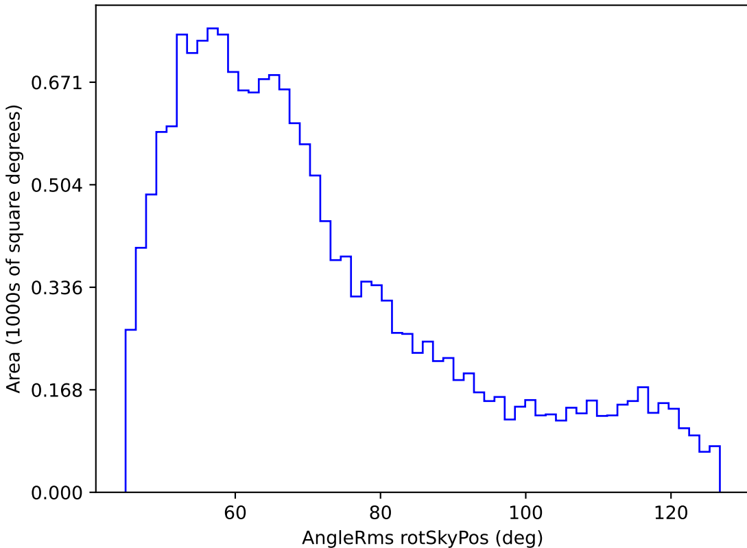
baseline_v3.5_10yrs WFD g band: AngleRms rotSkyPos
