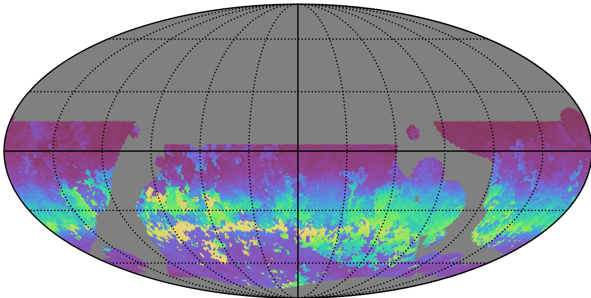
baseline_v3.5_10yrs WFD all bands: AngleRms rotSkyPos
