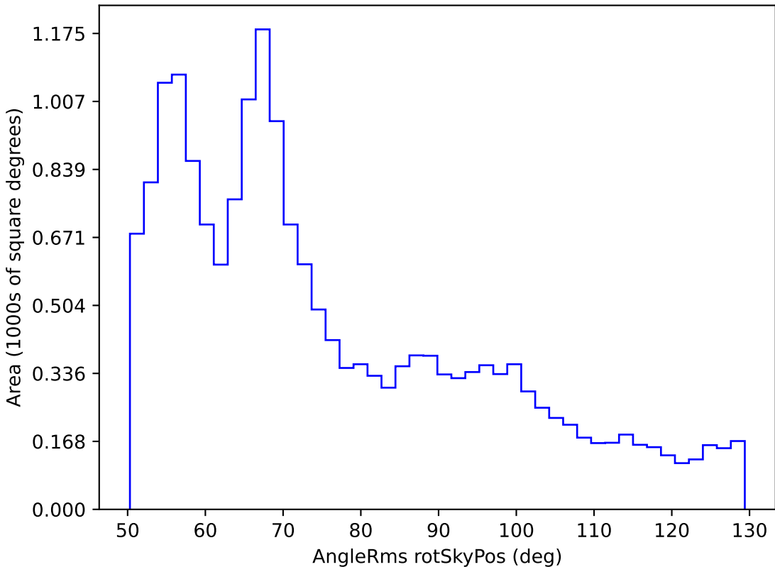
baseline_v3.5_10yrs WFD all bands: AngleRms rotSkyPos
