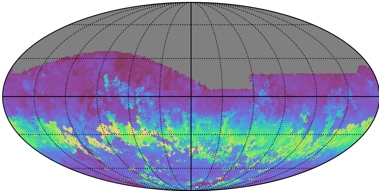
baseline_v3.5_10yrs All sky z band: AngleRms rotSkyPos
