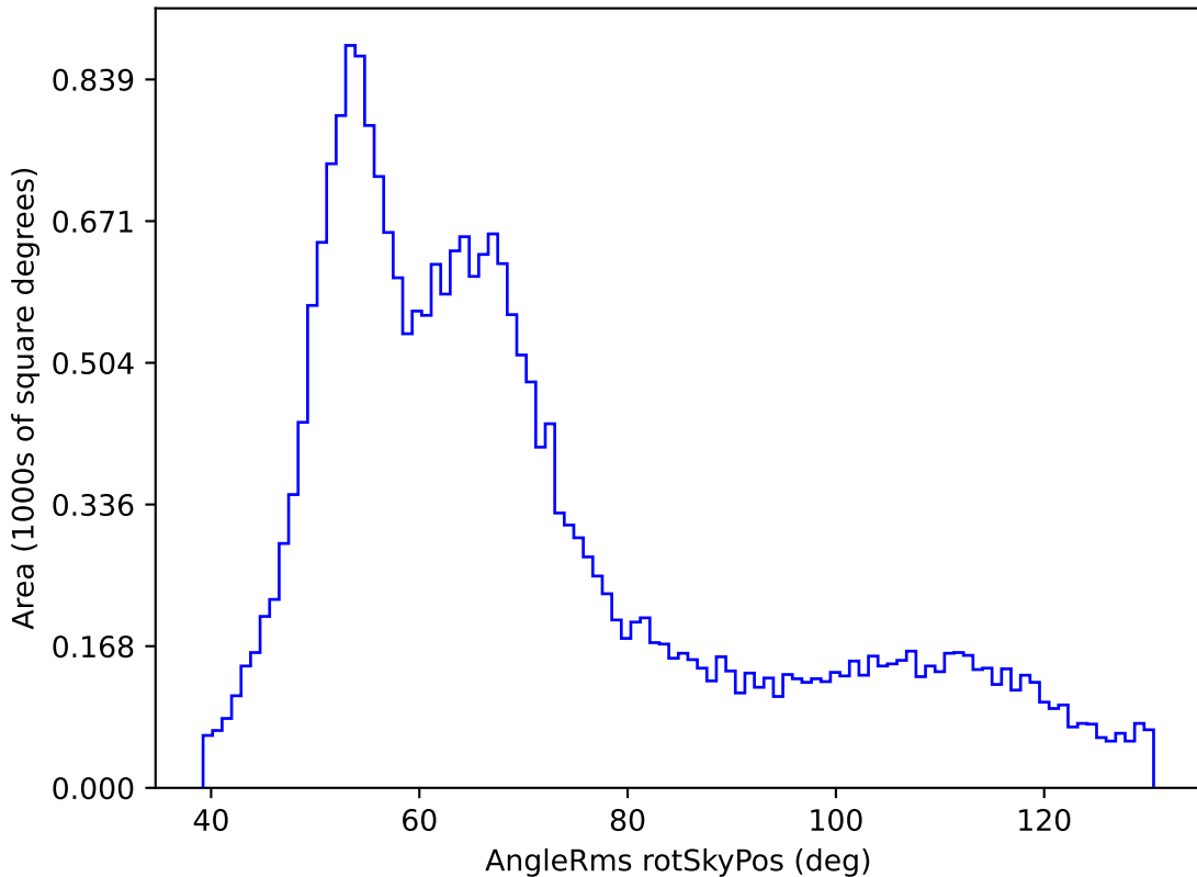
baseline_v3.5_10yrs All sky z band: AngleRms rotSkyPos
