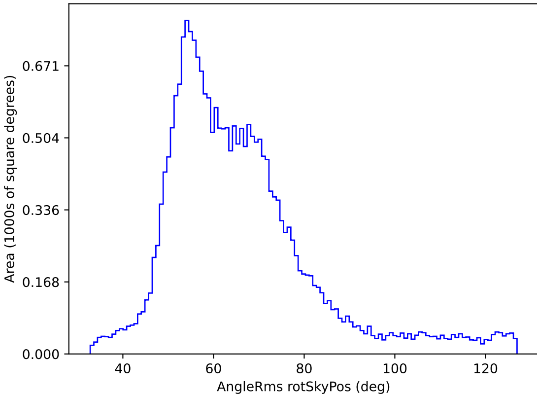
baseline_v3.5_10yrs All sky y band: AngleRms rotSkyPos
