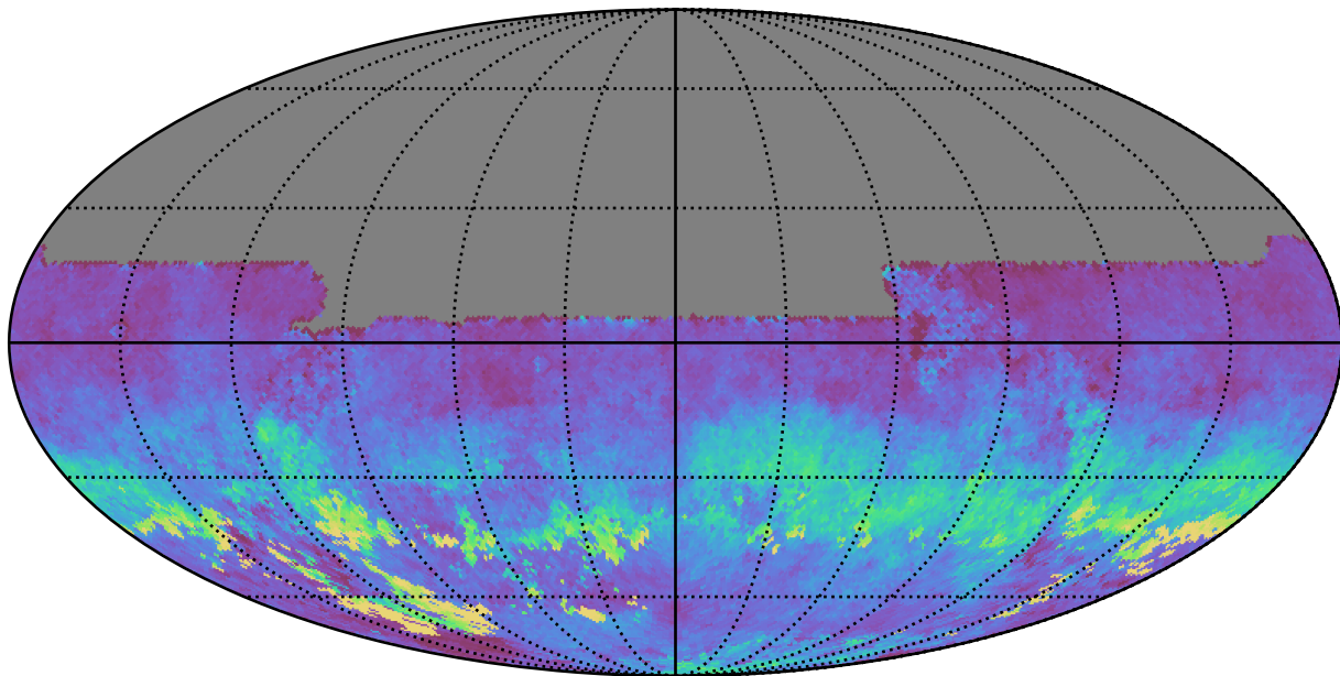
baseline_v3.5_10yrs All sky u band: AngleRms rotSkyPos
