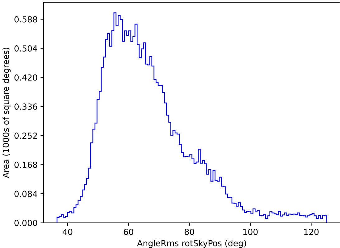
baseline_v3.5_10yrs All sky u band: AngleRms rotSkyPos
