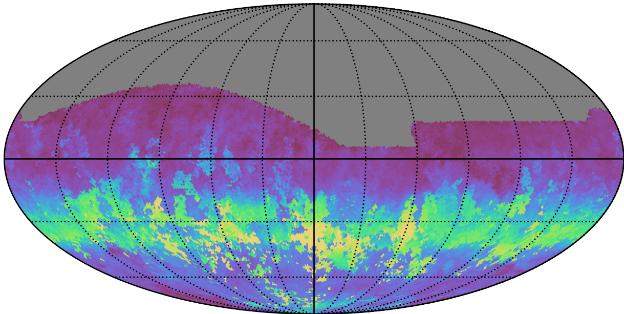
baseline_v3.5_10yrs All sky r band: AngleRms rotSkyPos
