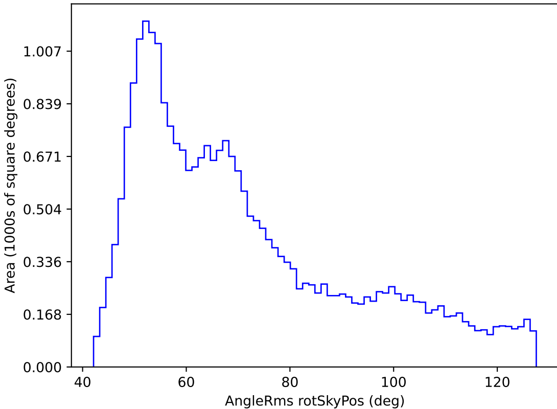
baseline_v3.5_10yrs All sky r band: AngleRms rotSkyPos
