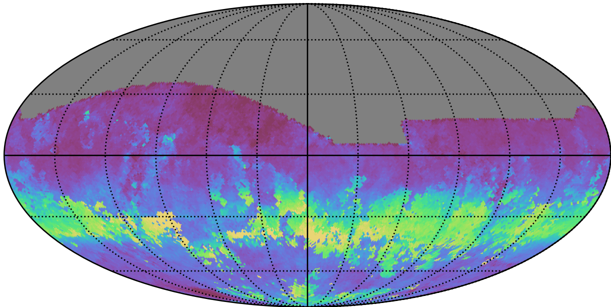
baseline_v3.5_10yrs All sky i band: AngleRms rotSkyPos
