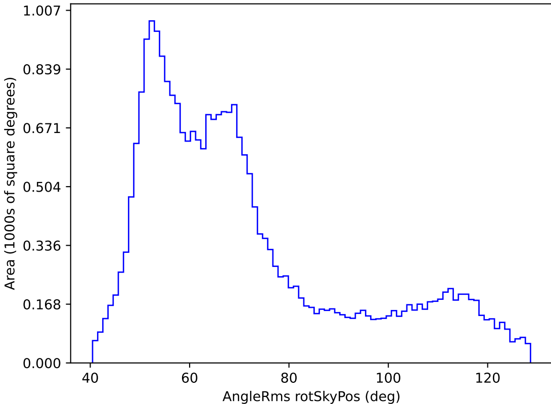
baseline_v3.5_10yrs All sky i band: AngleRms rotSkyPos
